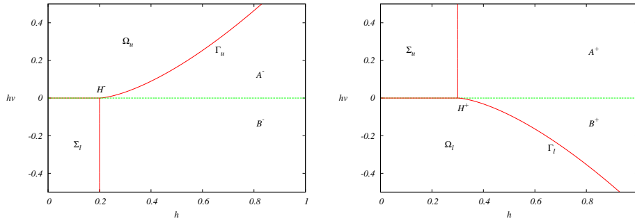
FIGURE 3. Representation of the regions introduced in Lemma 2.2
