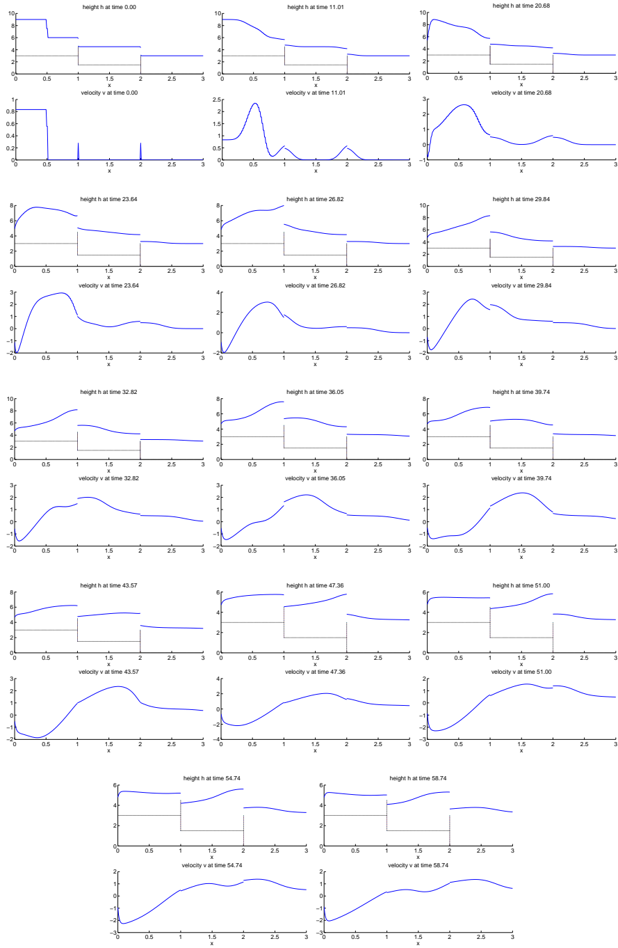
FIGURE 6. Simulation results for a strong wave entering the pooled step. Initially, the water level on each step is above the critical level. The solution (h, v) at different times is depicted. The time increases from left to right and top to bottom.
