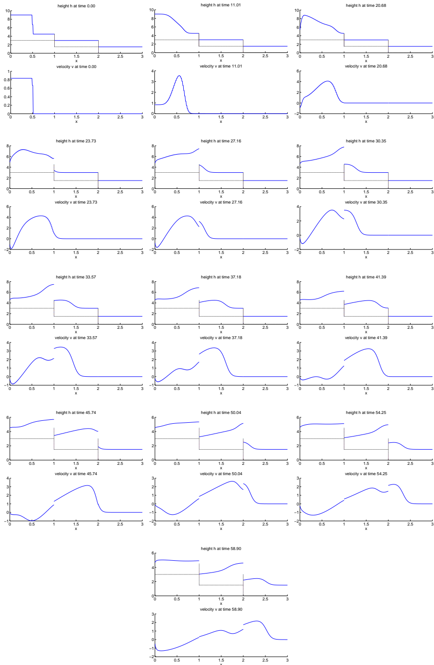
FIGURE 5. Simulation results for a strong wave entering the pooled step. Initially, the water level on each step is below critical. The solution (h, v) at different times is depicted. The time increases from left to right and top to bottom.
